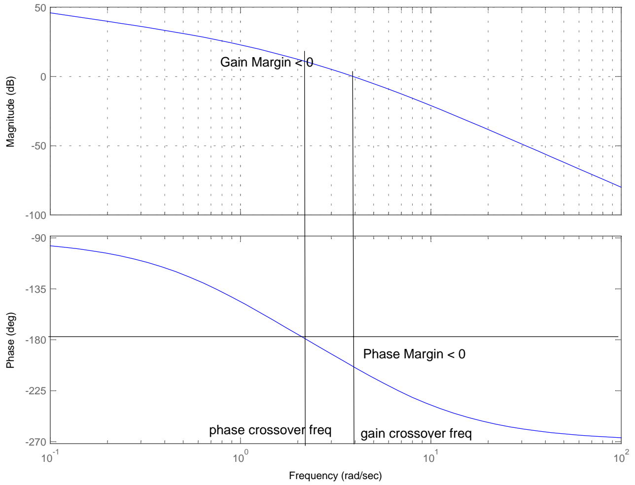
Bode Plot with Gain K=100
